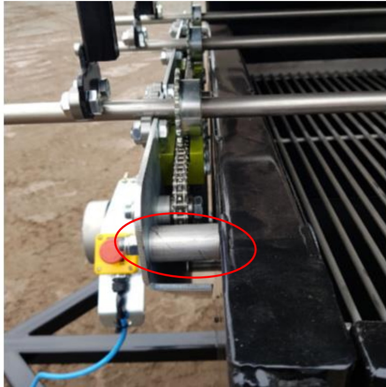
Image 6 Plate retainer system
